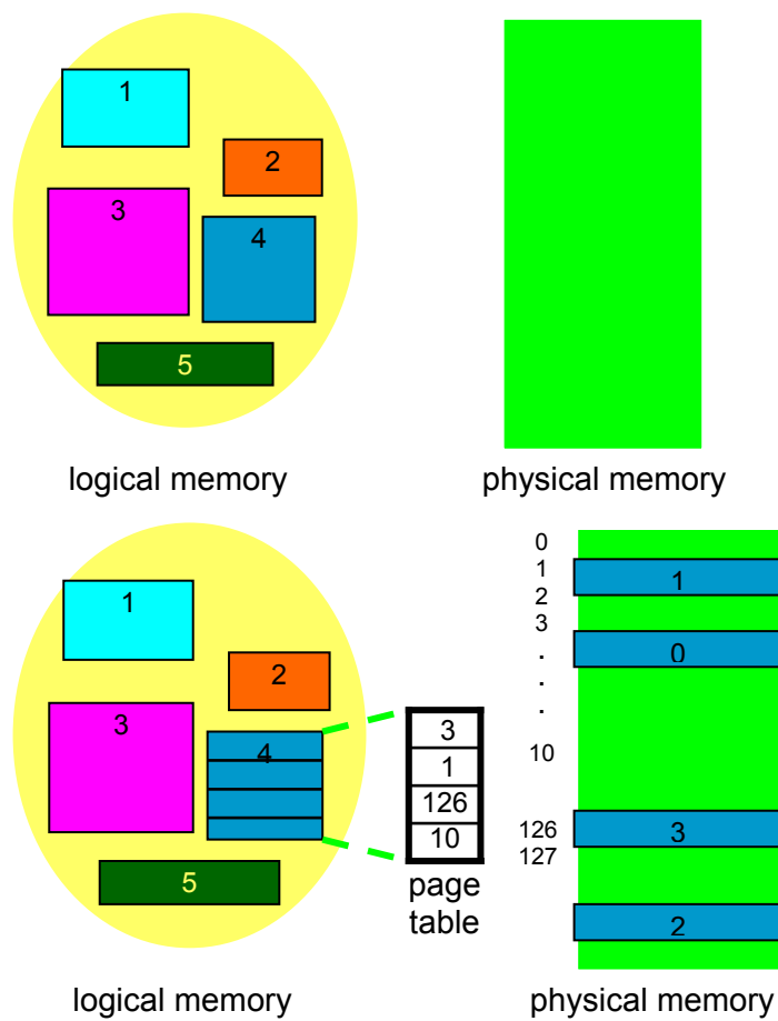
Paged Segmentation
